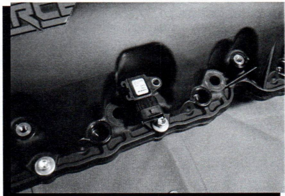
Figure 8 Install the MAP Sensor.
