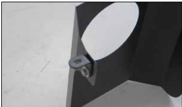
10. Install the "L" bracket (070066) onto the heat shield with the provided hardware through the non-slotted hole in the bracket.
