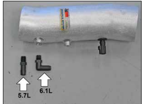
18. Install the appropriate 1/4npt fitting into the K&N® intake tube. The 90° fitting is for 6.1L engine size and the straight fitting are for 5.7L engine size. On 5.7L equipped vehicles, it will be necessary to choose either 1/2" and 5/8" CCV hose and fitting to install into the K&N intake tube depending on the size of the factory CCV hose. NOTE: Plastic NPT fittings are easy to cross thread. Install the vent fitting "hand" tight, then turn it two complete turns with a wrench.
