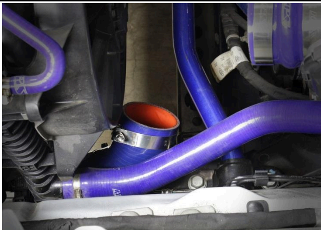
20. Insert the 45 degree coupler along with the t-bolt clamps onto the intercooler outlet.
