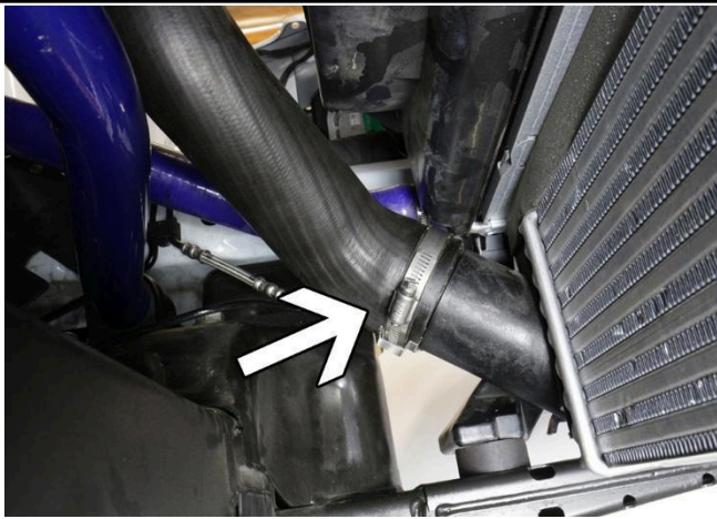
10. Loosen the lower hose clamp that's connected to the intercooler and remove the hose from the vehicle.
