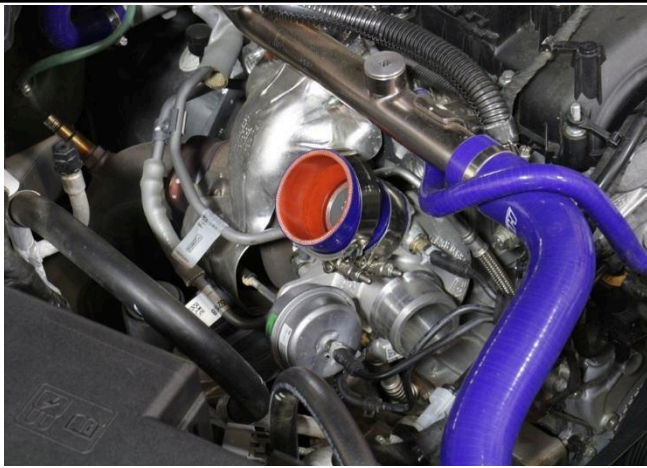
16. Insert the provided reducer coupler onto the turbo outlet along with the T-bolt clamps.
