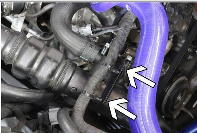
14. Remove the two clips that are holding the wiring harness attached to the hot pipe assembly, Unplug the BPV wiring, then remove the hot pipe from the vehicle.
