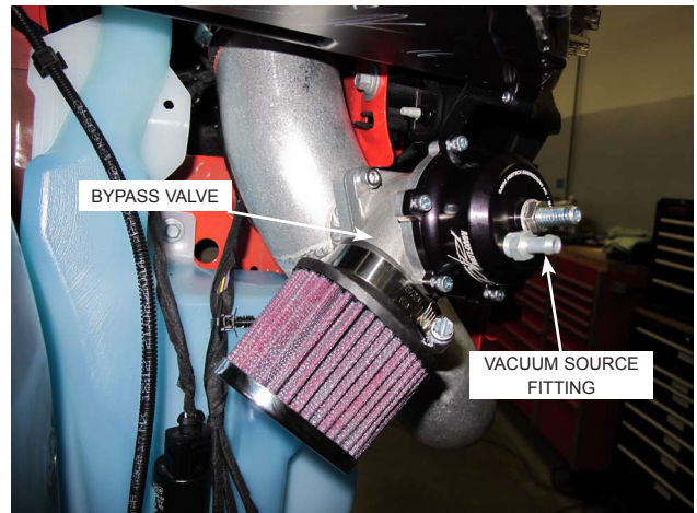
Fig. 9-d: Bypass Valve
