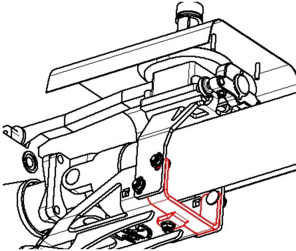
FIG 5-Final Assembly with Extension Bracket (V6 & Ecoboost)
