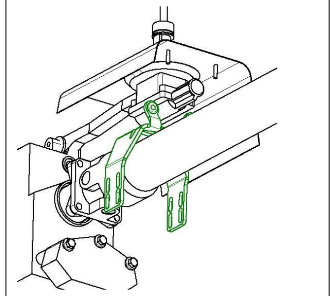
FIG 2-Upper Bracket Placement
