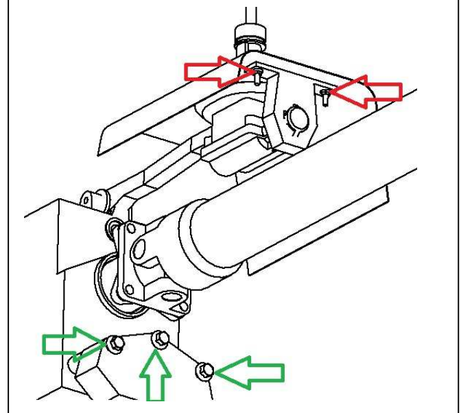
FIG 1-Rear Shifter Mount and Trans Isolator Bolts
