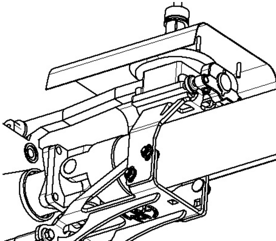
FIG 6-Final Assembly without Extension Bracket (V8)
