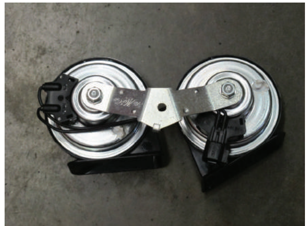
Fig. 6B: Modified Horn Bracket Orientation
